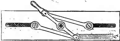
Fig. 65.—KINNE'S TURN-TABLE. (Under side.)
